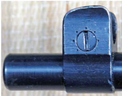
The left-hand side of the M39 front sight assembly. Note dots embossed into the front sight base surrounding the windage adjustment screw allowing for precise zeroing.
