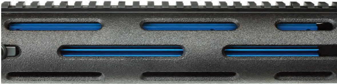
Top, the SCR-11 receiver. Above, left side profile of the SCR-11. Note the blue aluminum radiator on the barrel. Below, a close up of the aluminum radiator.
