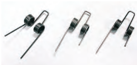
Three failed hammer springs. From left to right, uneven hammer spring leg tension, one bent leg and one broken leg, and one with one broken leg. All can result in malfunctions.
