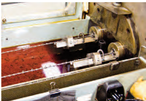
This station is a broaching machine for rifling pistol barrels.
